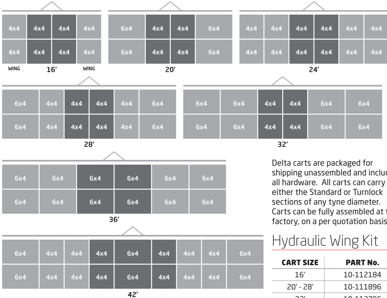
Cart and section configurations (in feet)
